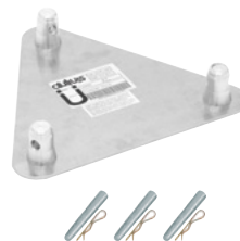
No. 6030189A No. 6030189B..... with connector set ALUTRUSS TRILOCK Base/Wall-Plate QTG-male
