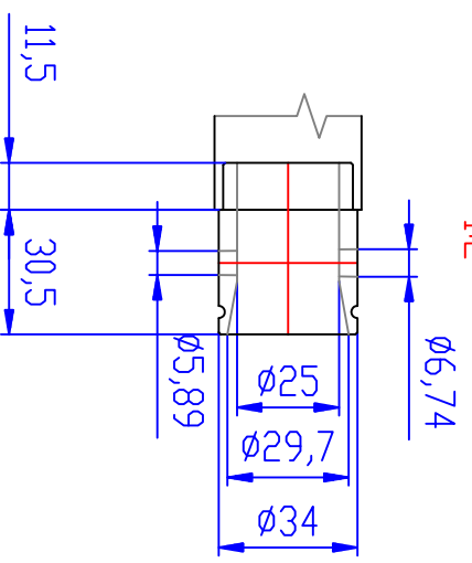
DETAIL A 1:2
