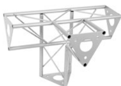
DECOTRUS SAT-42 4-way piece V No. 60112244 ..... 2.1 kg
