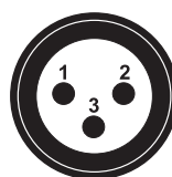
DMX-input XLR mounting-plug:
