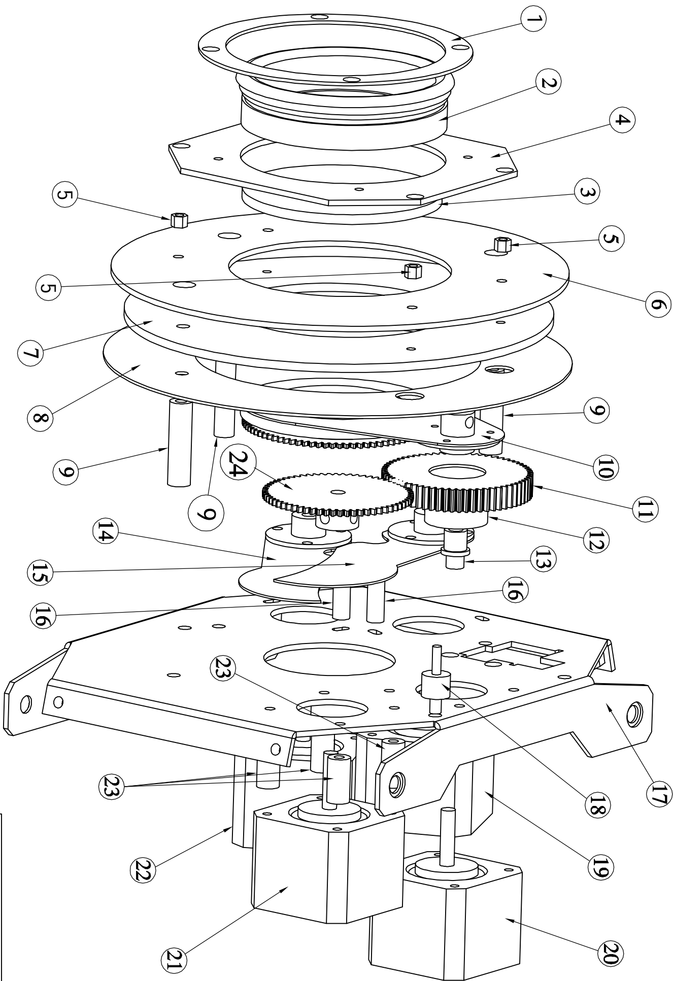
FUTURELIGHT DJ-Head 575 Spot
