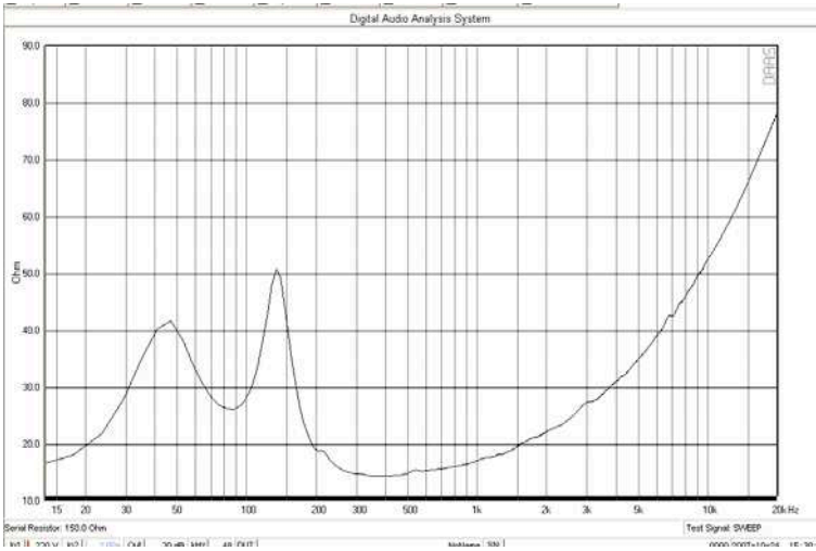
Impedance Curve
