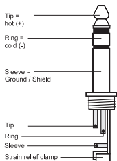
Balanced use of 6.3 mm jack plugs
