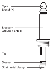
Unbalanced use of 6.3 mm jack plugs
